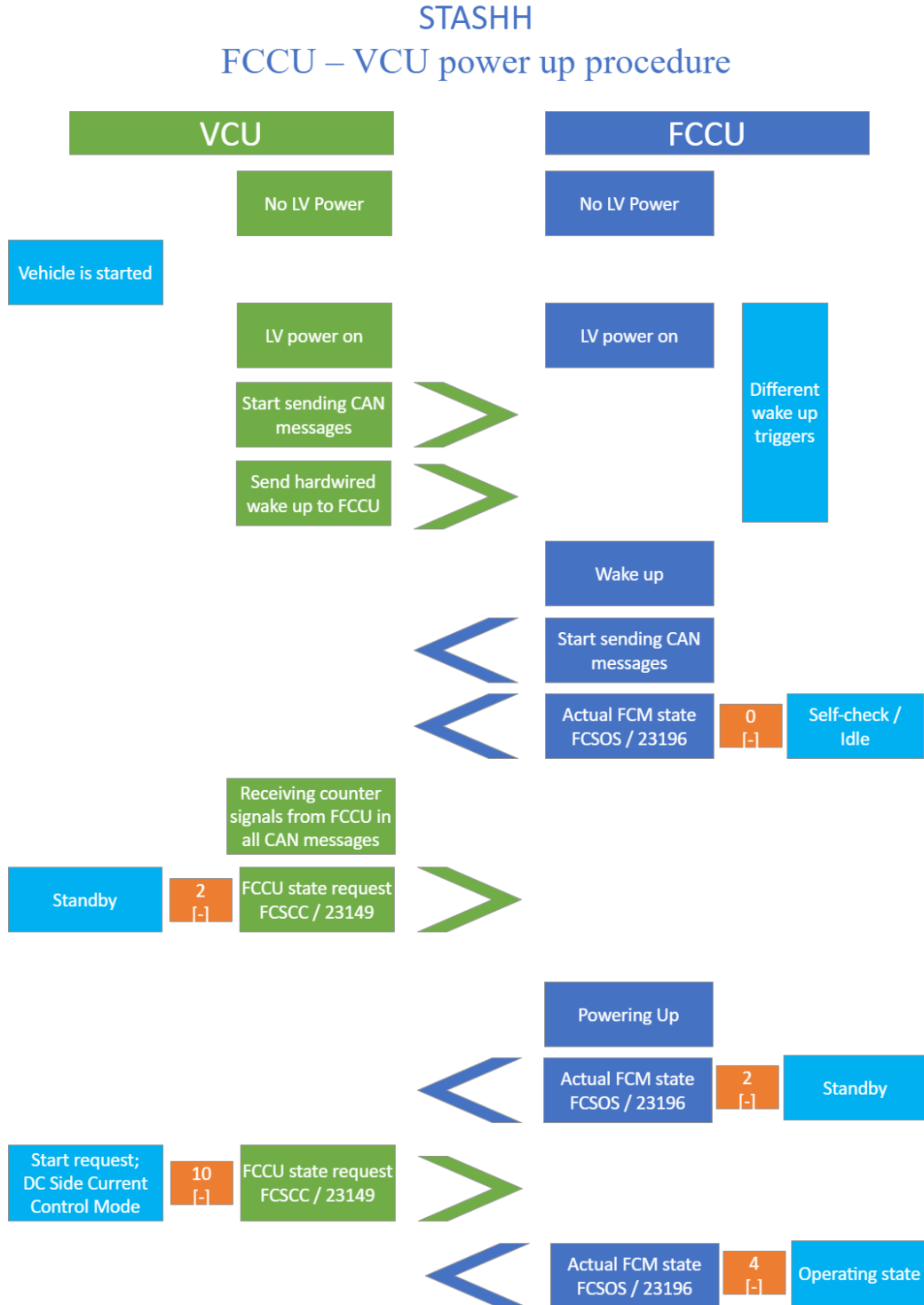
Figure 21. Startup procedure.
